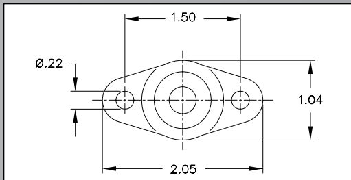
Heavy Duty Die Cast Base Adjustable Position Swivel
