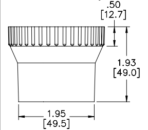
1984 2" Lock Ring w/2" Hose Adapter
