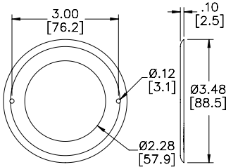
2030 2.25" Cover (Screw Mount Option)
