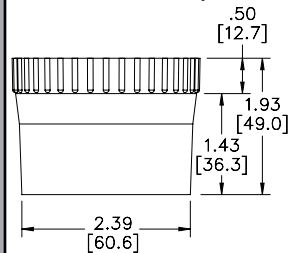
1993 2" Lock Ring w/2.5" Hose Adapter
